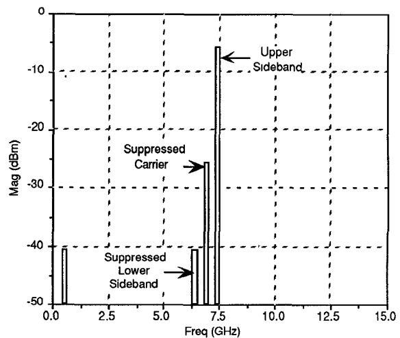
Figure 6. Frequency Spectrum of the Single Sideband Modulator Output Port
