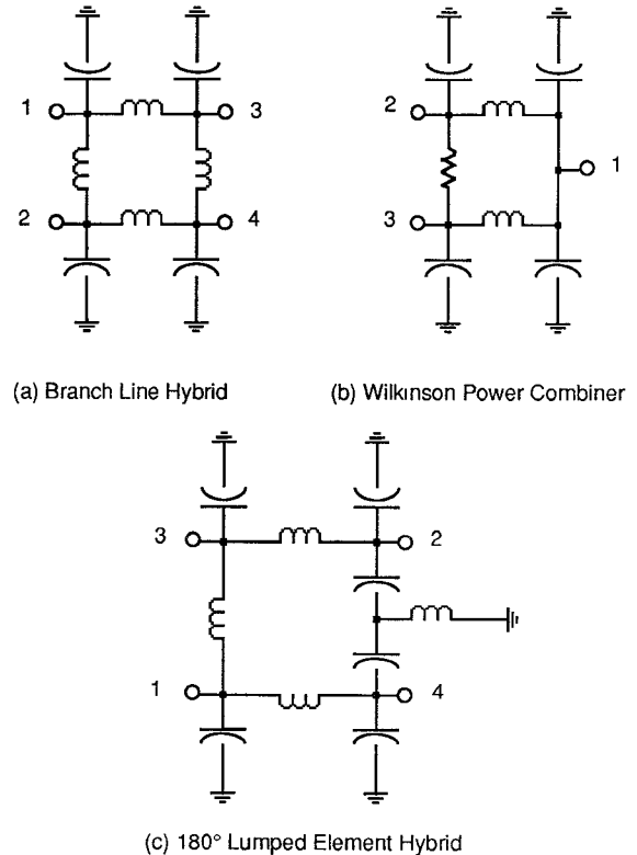
Figure 2. Schematics of the Lumped Element Circuits
